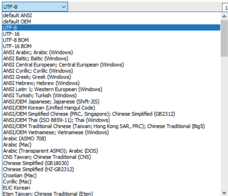
Fig. 13: Encoding with UTF-8
